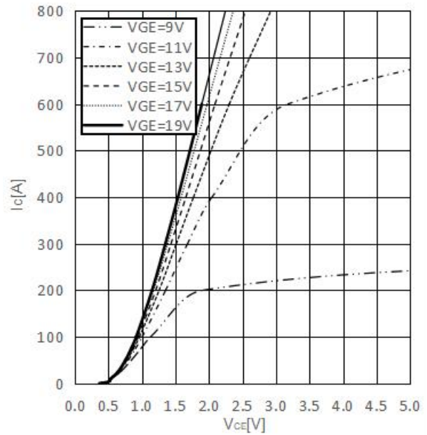
Output characteristic IGBT, Inverter (typical), Inclusive R_{CC+EE} IGBT 输出特性, 逆变 (典型值), 包含 R_{CC+EE} I_c = f(V_{CE}), T_{vj} = 150^\circ\text{C}
