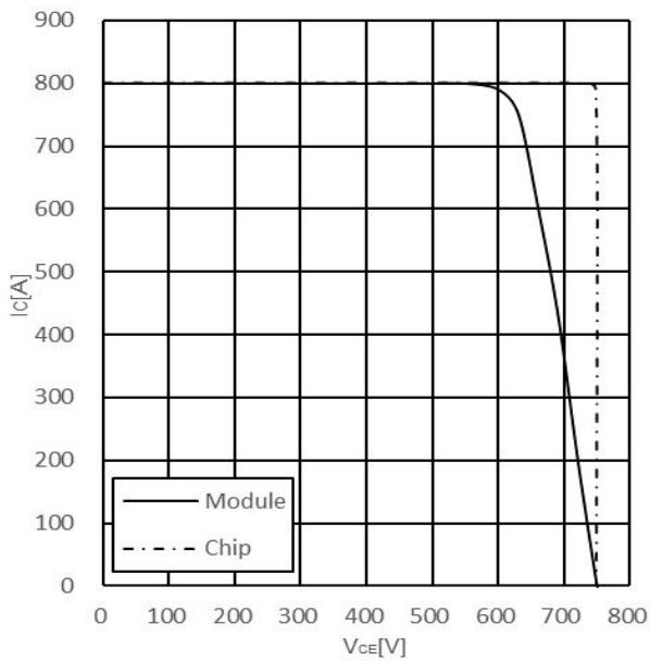
Reverse bias safe operating area IGBT, Inverter (RBSOA) IGBT 反向安全工作区, 逆变 (RBSOA) I_C=f(V_{CE}), V_{GE}=+15V/-8V, R_{Goff}=10\Omega, T_j=150^\circ C
